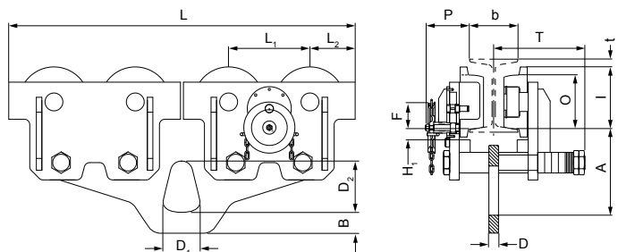
Model HTG, 50000 kg
