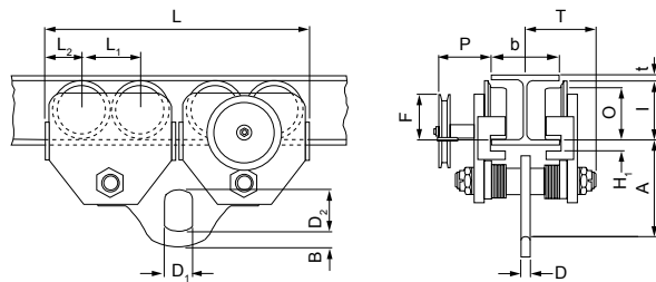
Model HTG, 20000 kg
