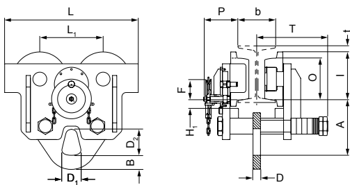
Model HTG, 30000 kg
