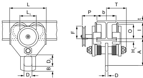
Model HTG, 10000 kg
